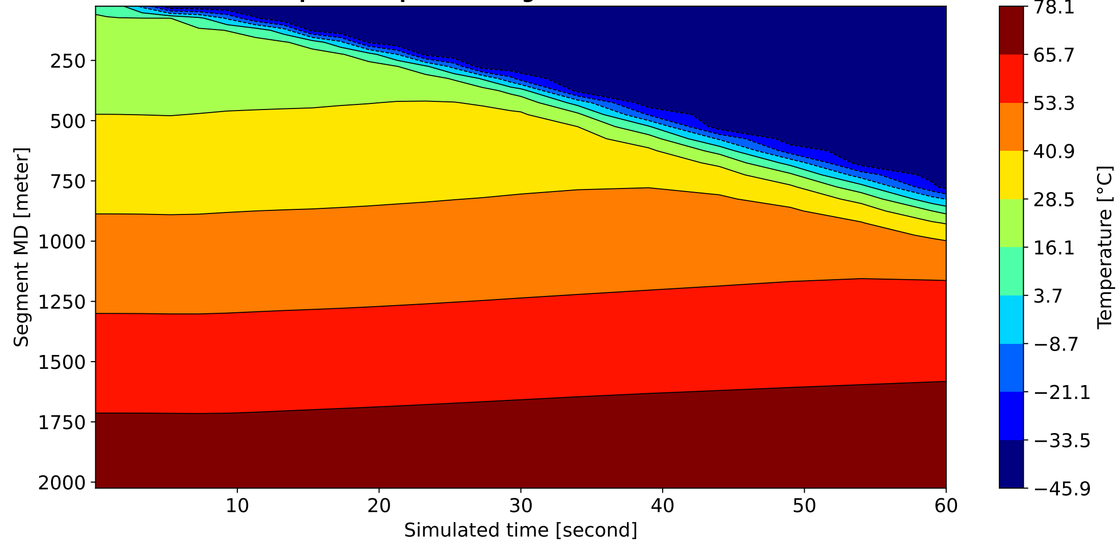
Temperature profile along the wellbore over time
